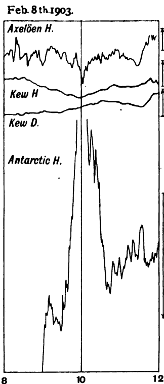
FIG. 38. ARCTIC-KEW-ANTARCTIC CURVES.
